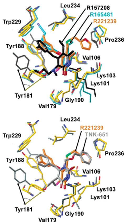
Figure 2. Inhibitor conformations in the NNIBP. The figure was generated using the program Maestro. 51 (a) (Upper panel) The superposition of the structures of the three RT/NNRTI complexes is shown (R157208 carbons in black, R165481 carbons in cyan, R221239 carbons in orange, RT/R221239 protein carbons in yellow). For clarity, Pro95, Leu100, Phe227, and Tyr318 are not shown. The benzyl/phenoxyl ring (left) is in the wing I position (using the butterfly-like analogy 24,52 ), and the pyridinone ring (right) occupies the wing II position. To accommodate the (2-methoxyethyl)methylamino substituent of R157208, the Tyr181 side chain is rotated (upward) toward Trp229 in the RT/R157208 complex compared to the other two complexes. (b) (Lower panel) Superposition of RT/R221239 and RT complexed with HEPT-like TNK-651 (gray). If the isopropylpyrimidine ring of TNK-651 is replaced with the iodopyridinone ring of R221239, the Tyr181 side chain is not flipped.
